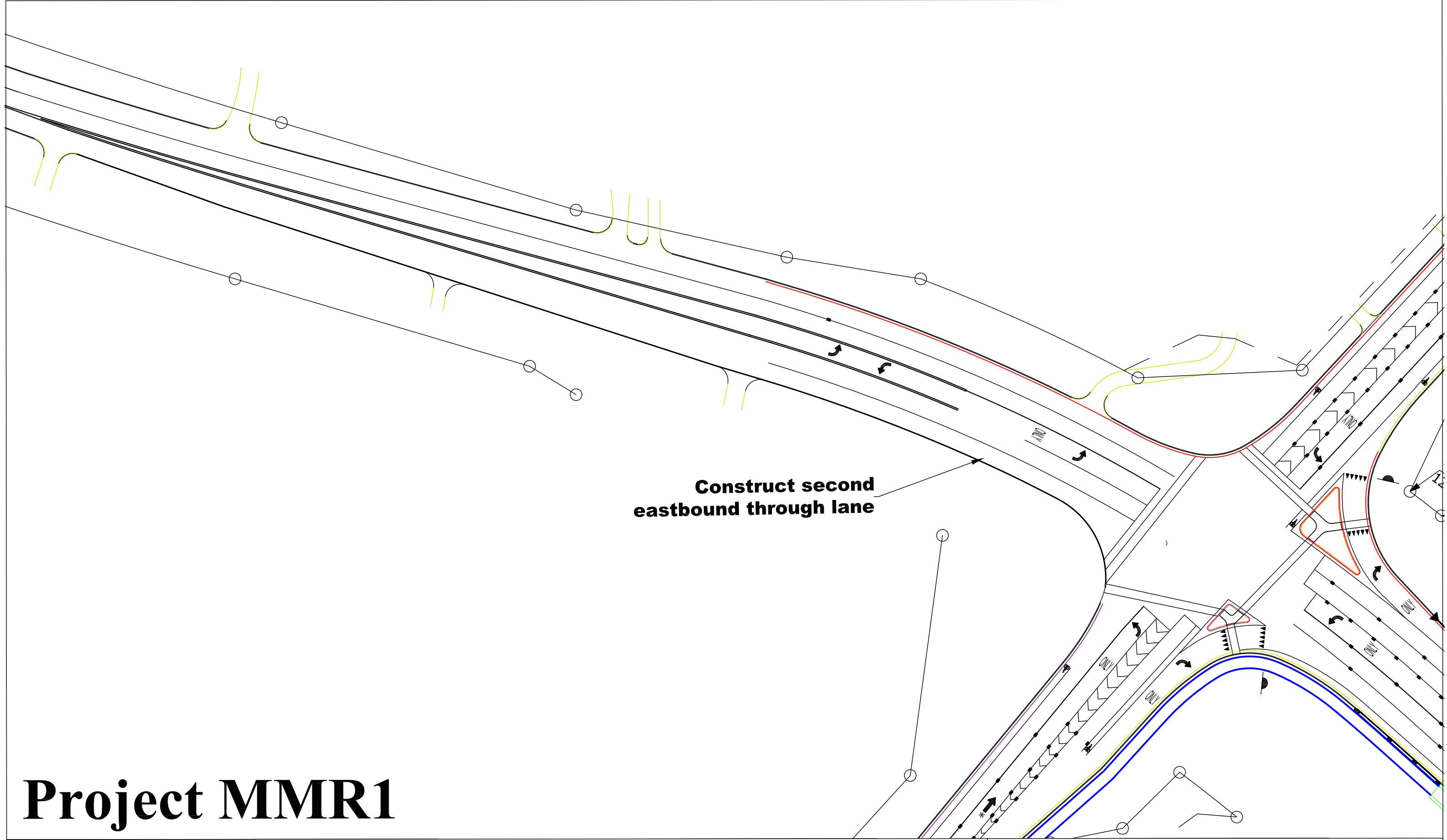
Figure 4 - Moore Mill Rd at E. University Drive Future Improvements Auburn, Alabama
