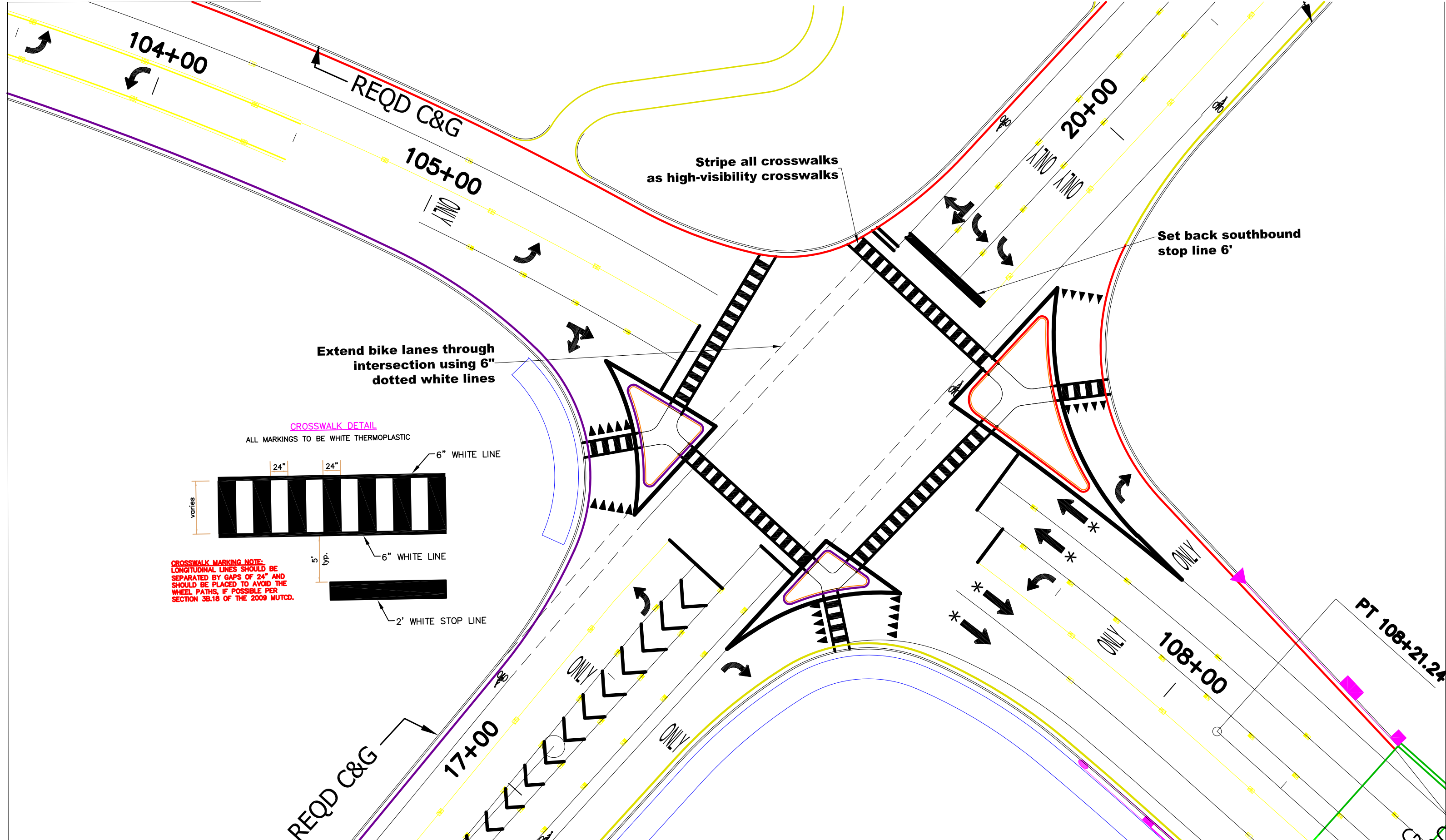
Figure 5 - Moore Mill Rd at E. University Drive Existing Improvements Auburn, Alabama
